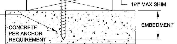
VERTICAL SECTION B-B
