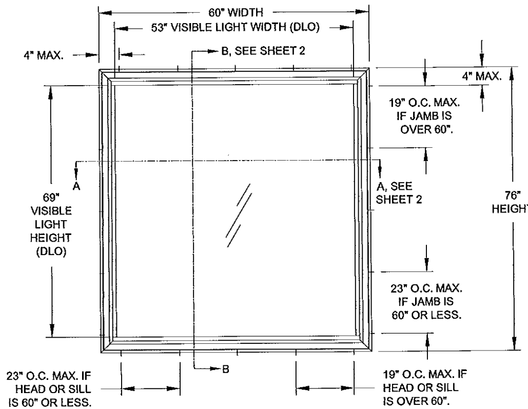
TYP. ELEVATION OF FIXED CASEMENT WINDOW
