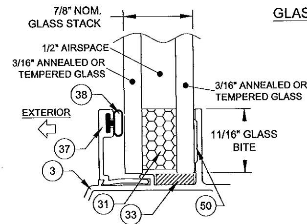
GLASS TYPES 9 & 10
