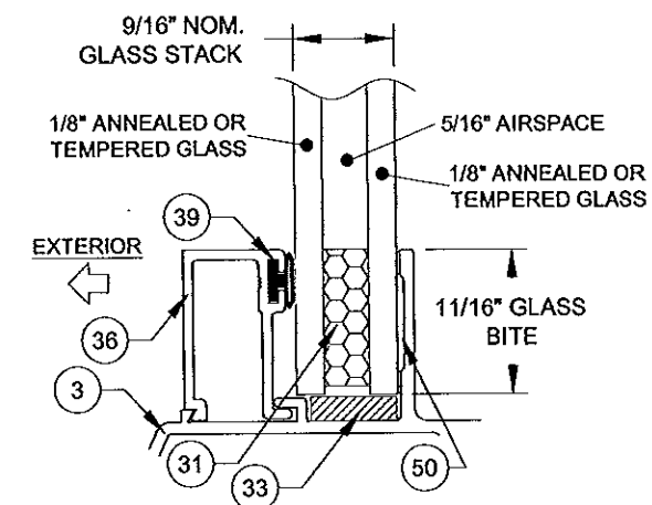
GLASS TYPES 7 & 8
