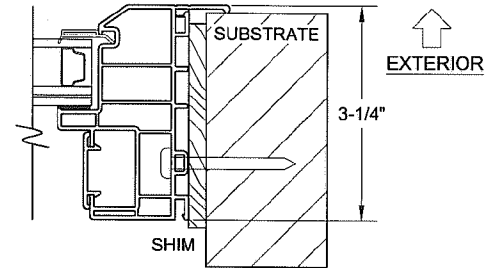
FLANGE FRAME, JAMB INSTALLATION (DIRECTLY TO SUBSTRATE)
