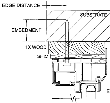
FLANGE FRAME, HEAD INSTALLATION (USING 1X BUCKSTRIP)
