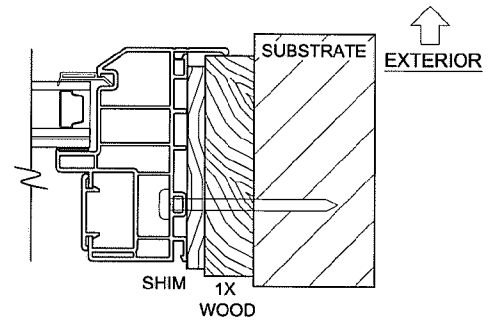
FLANGE FRAME, JAMB INSTALLATION (USING 1X BUCKSTRIP)
