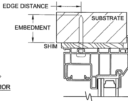
FLANGE FRAME, HEAD INSTALLATION (DIRECTLY TO SUBSTRATE)
