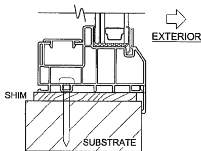
FLANGE FRAME, SILL INSTALLATION (DIRECTLY TO SUBSTRATE)
