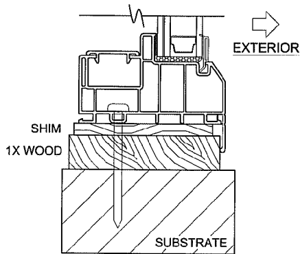
FLANGE FRAME, SILL INSTALLATION (USING 1X BUCKSTRIP)
